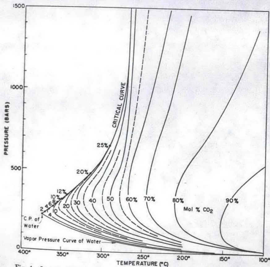
Fig. 4. Isocompositional curves of the gas phase in equilibrium with the liquid phase in the system H_2O-CO_2 .
