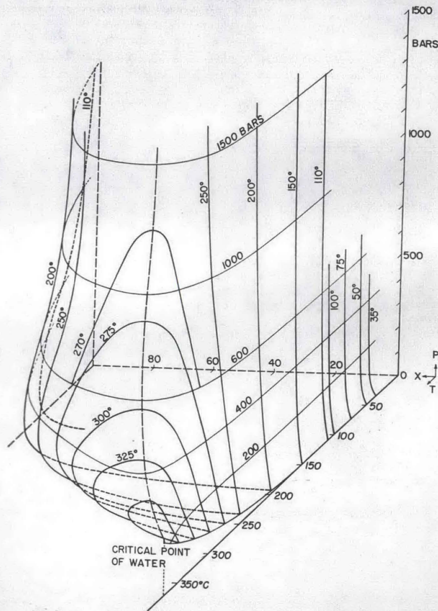
Fig. 6. Temperature-pressure-composition diagram of the system \text{H}_2\text{O}-\text{CO}_2 .
