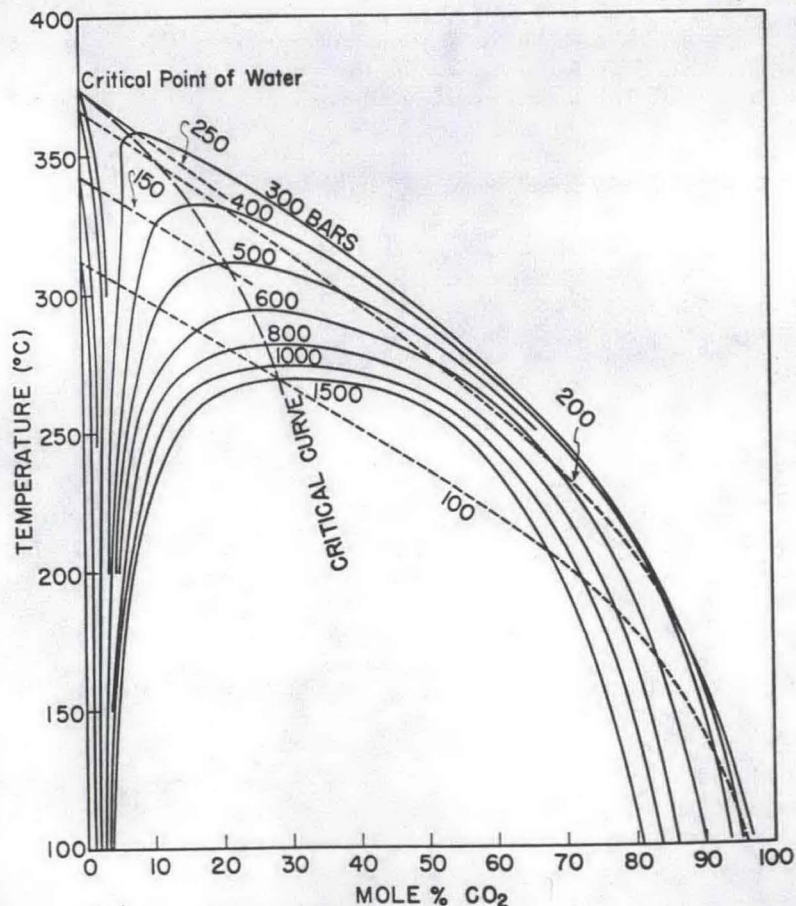
Fig. 3. Isobaric curves with the critical curve for the system H_2O-CO_2 .
